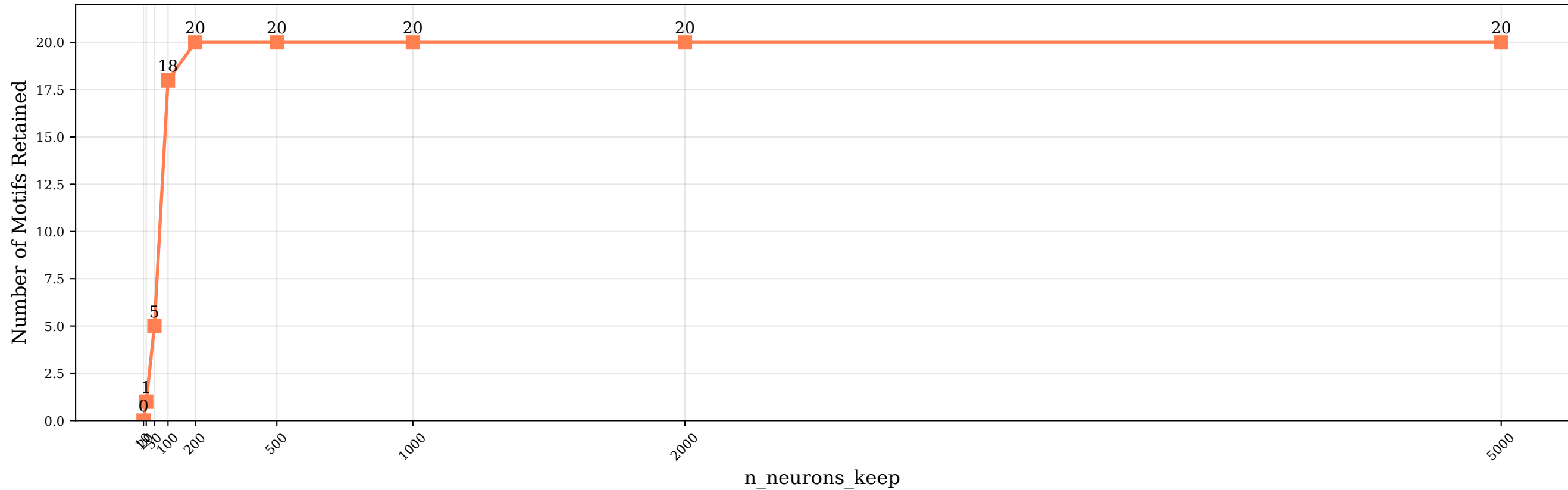
Motif Retention vs Neuron Threshold sigma: (0.02, 0.4) | volume: (0.03, 0.9)
